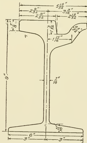
Fig. 225. "Trilby" or Grooved Rail
